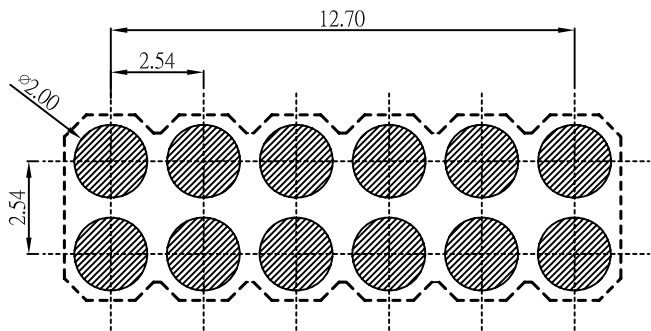
Recomended pcd layout layongt tolerance: ±0.05mm
