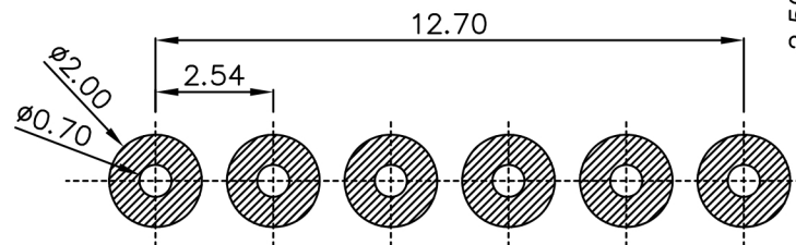
Recommended pcb layout Layout tolerance: ±0.05mm
